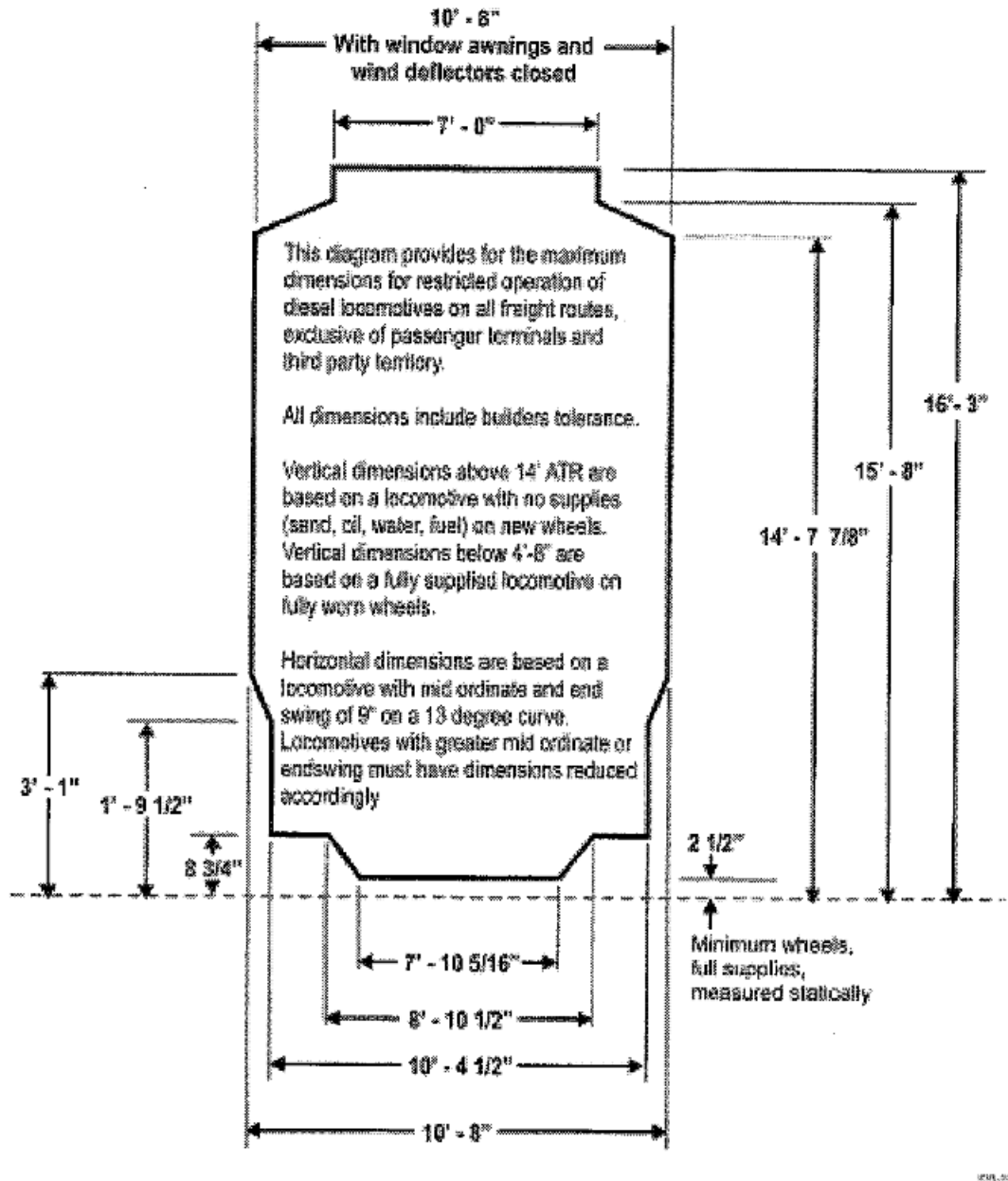
Fig. 2.1 Freight locomotive Plate L
