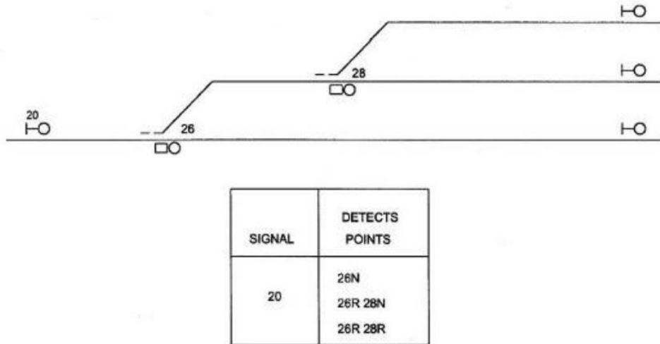
Figure 11 Detection of Facing Points in Routes
