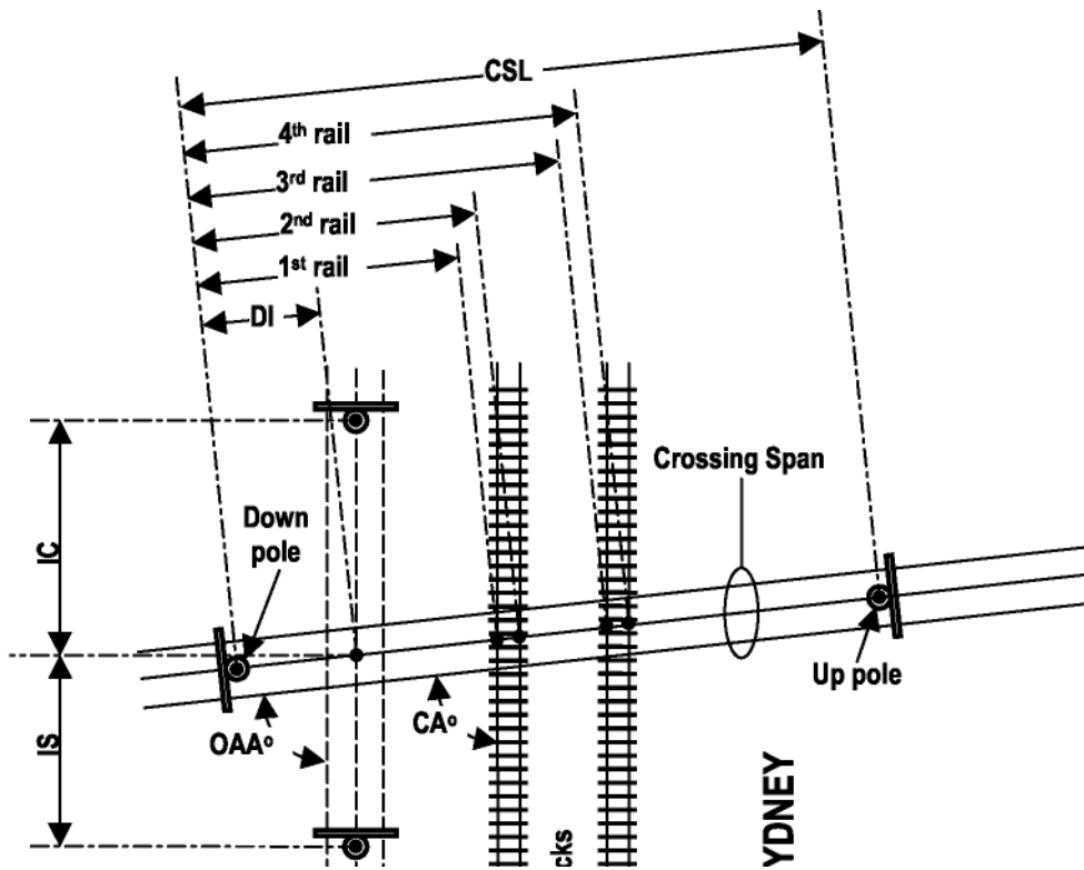
Diagram 1 – Electric aerial crossing plan
