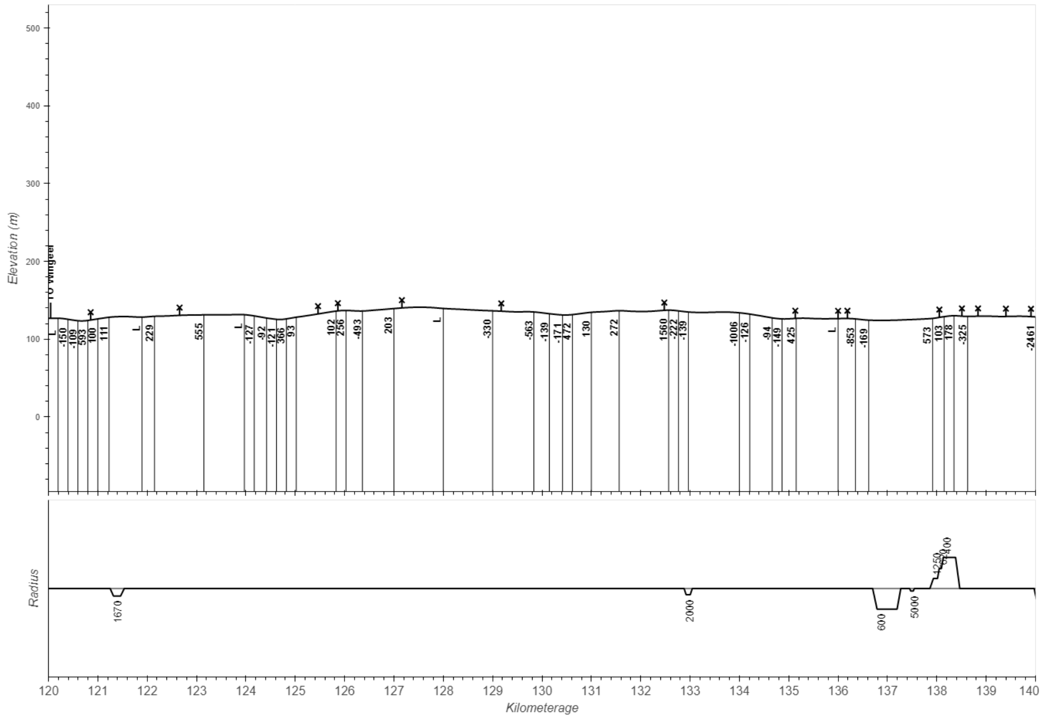
V01 - Tottenham to SA Border: 120 to 140 kms
